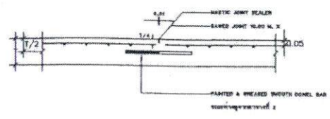
CONTRACTION JOINT
