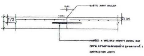
CONSTRUCTION JOINT
