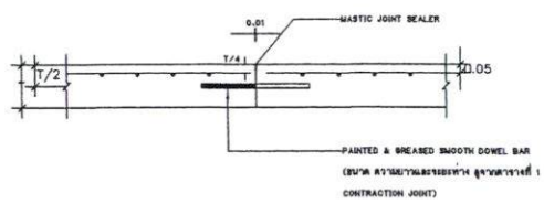
CONSTRUCTION JOINT
