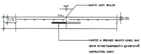
CONSTRUCTION JOINT
