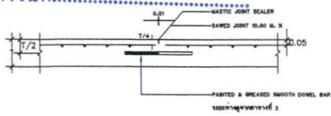
CONTRACTION JOINT
