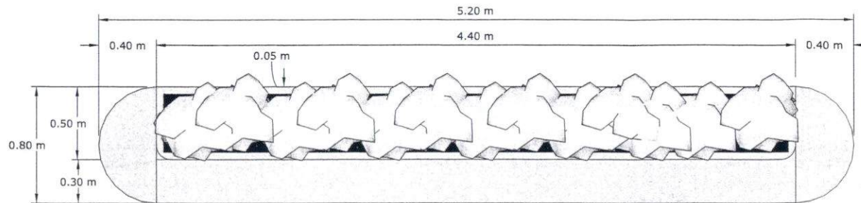
Plan
