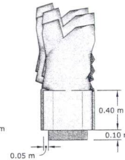
Left Elevation
