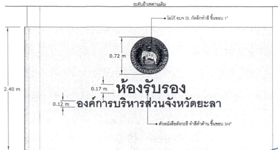
Front Elevation
