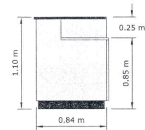
Left Elevation
