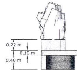
Left Elevation
