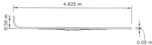
Plan
