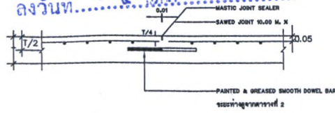
CONTRACTION JOINT
