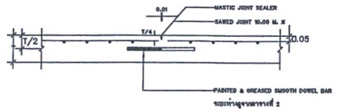
CONTRACTION JOINT
