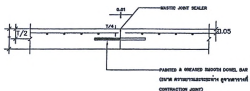
CONSTRUCTION JOINT
