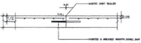
CONSTRUCTION JOINT
