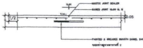
CONTRACTION JOINT
