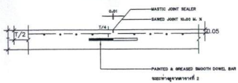
CONTRACTION JOINT
