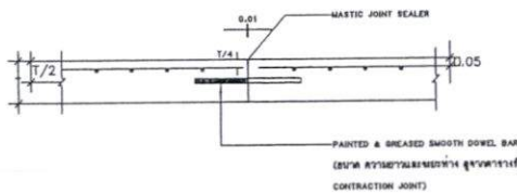
CONSTRUCTION JOINT
