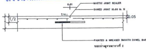
CONTRACTION JOINT
