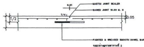
CONTRACTION JOINT
