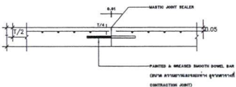
CONSTRUCTION JOINT
