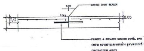
CONSTRUCTION JOINT
